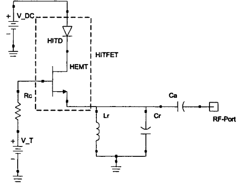
Fig. 3: HITFET based VCO circuit schematic
